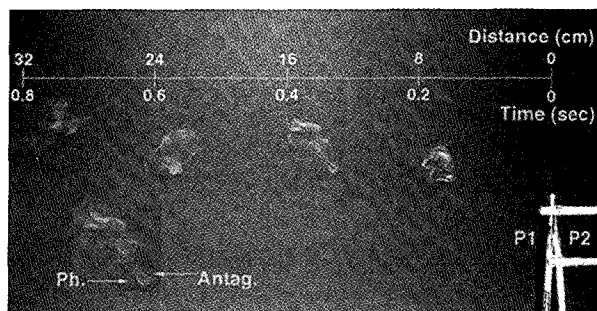
Figure 4. Smoke visualization of how two strands of odour would look emerging from pipette tips (P1 and P2) stationed only 1 mm apart, a distance over which Helicoverpa zea can discriminate strands of pheromone from strands of antagonist. Abbreviation used: Ph., pheromone; Antag., antagonist (see ref. 6).
