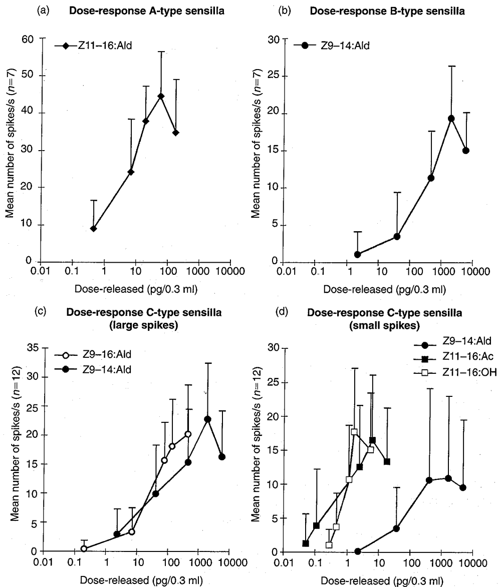
Figure 2. Sensitivities of the neurons in the three different sensillar types to their respective optimal odourants. Note that in sensillar type C, the large-spiking agonist-related neuron (c) is equally sensitive to Z9-16:Ald and Z9-14:Ald and that the small-spiking neuron (d) is optimally sensitive to Z11-16:Ac and Z11-16:OH, both of which are known behavioural antagonists. This neuron also responds to Z9-14:Ald, but any behavioural antagonism would come at a slightly higher airborne concentration than attraction, due to stimulation of the large-spiking neuron in the same way (see ref. 6).
