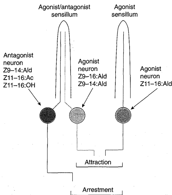
Figure 3. A depiction of the relationship of sensillar types A (right) and C (left) to upwind flight attraction (agonism) and arrestment (antagonism) in Helicoverpa zea males. Attraction occurs when the pheromone components Z11-16:Ald and Z9-16:Ald stimulate the respective neurons that are tuned to them. If the small-spiking neuron in sensillar type C is stimulated, upwind flight is reduced by the increasing amount of activity in this neuron until arrestment of flight predominates.
