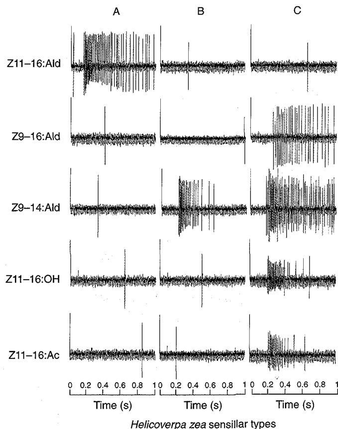
Figure 1. Sensillar types A, B and C on Helicoverpa zea male antennae contain neurons tuned to different pheromone-related components. Type A always contains a large-spiking neuron related to attraction (agonism) tuned to Z11-16:Ald. Type B contains neurons tuned only to Z9-14:Ald, which is a component emitted by Heliothis virescens (not Helicoverpa zea ) females. Type C contains a large-spiking agonistic-related neuron tuned equally to the Helicoverpa zea pheromone component Z9-16:Ald and to Z9-14:Ald. Type C also contains a small-spiking neuron related to antagonistic behavioural response that is tuned to Z11-16:Ac and Z11-16:OH, but also has some sensitivity to Z9-14:Ald (From ref. 6).
