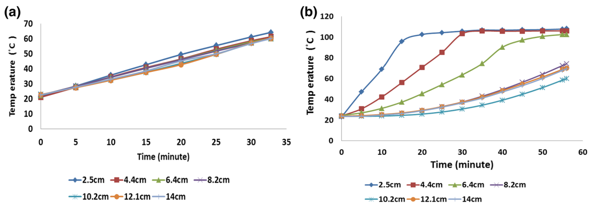
Fig. 6 Temperature evolution at different depths of 25 × 25 cm 2 wood specimens during a EPRF or b MW heating
