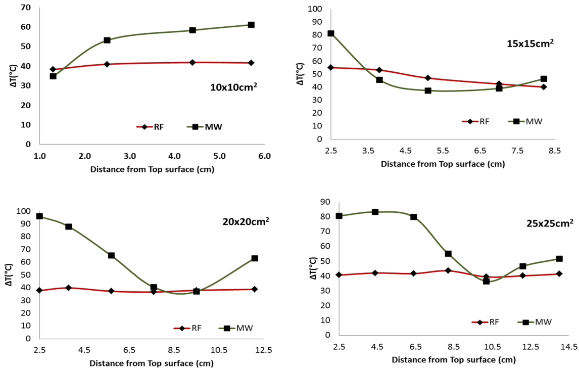
Fig. 5 Mean temperature increase ( \Delta T ) as a function of depth as measured from the top surface of green wood specimens (60–70 % MC) of a 10 × 10 cm 2 , b 15 × 15 cm 2 , c 20 × 20 cm 2 , and
