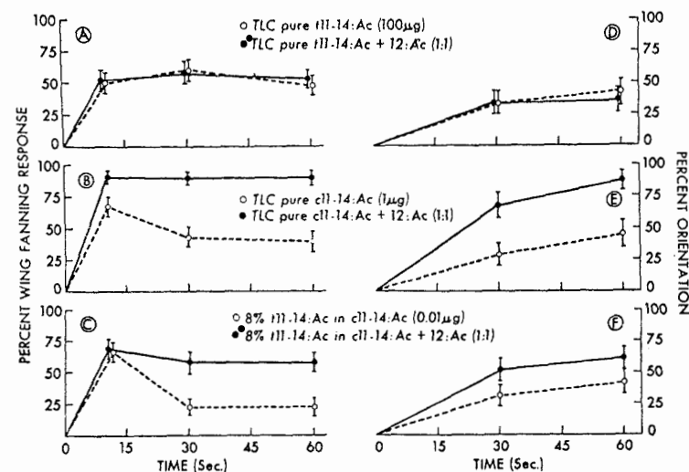
FIG. 3. Percentage wing-fanning response and orientation by A. velutinana males in glass tube olfactometers to mixtures of c11- and t11-14:Ac and 12:Ac at dose levels eliciting 50% response in box olfactometers. Brackets above and below the means denote the 95% binomial confidence limits ( n = 160 ).
