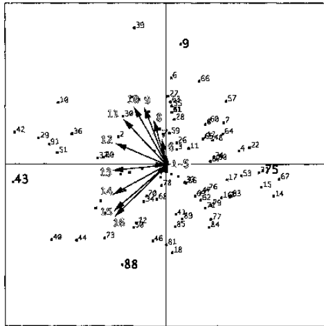
Figure 3. Biplot of the centred PCA of the table of spectral densities. The scatter plot is of the scores of the two principal eigenvectors. Each scatter point represent a unique time series. The four time series used as our main examples are indicated in bold face (nos. 75, 9, 43, and 88). Each arrow with associated contour text represents the standardized column scores of the spectral frequencies. The length of the arrow indicate the overall importance of this frequency in the ordination. The direction indicate how the frequency correlate with the principal components. The frequencies 1-6 are not very useful for discriminating the populations (the arrows have nearly no length). The second axis is positively correlated with the multiannual cyclic frequencies (7-10) and negatively correlated with the short term frequencies (14-16). The first axis is related to the overall average of each frequency ('the mean effect'). On the negative side the time series exhibit dominant frequencies in the inter-annual to multiannual cyclic frequencies, whereas on the positive side these frequencies are relatively unimportant.
