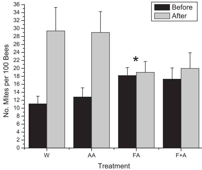
Fig. 3. Mean abundance of varroa mites (mean \pm SE) before and 4 wk after a 17-h treatment with a water control (W), acetic acid (AA), formic acid (FA), or both acetic and formic acids (F + A). An asterisk indicates a significant change in mean abundance of varroa mites in treated colonies compared with the change in mean abundance in the water control colonies ( P < 0.05 ).
